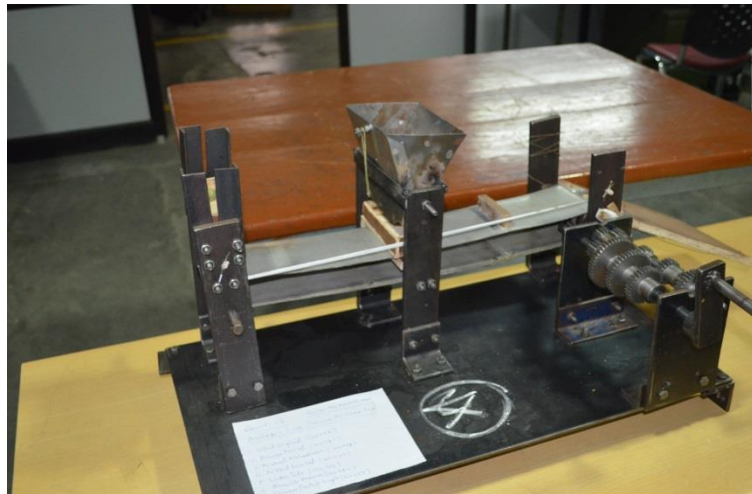
GROUP NO:56 ASSEMBLY LINE DRIVEN BY GEAR BOX SPECIAL APPRECIATION PROJECT
