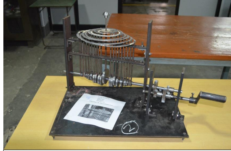
GROUP NO:64 WATER DROP EFFECTS 2 ND BEST PROJECT
