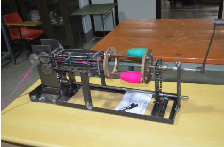
GROUP NO:5 FRENCH KNITTING MACHINE 1 ST BEST PROJECT
